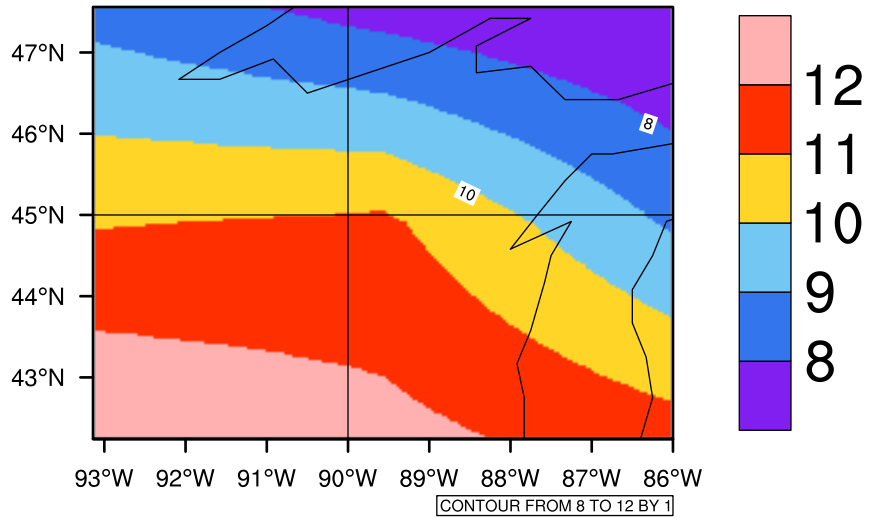
Yearly tasm max (c) In 2040-2049 GFDL-ESM2M RCP45 - Wisconsin
