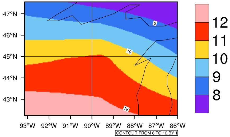
Yearly tasm max (c) In 2050-2059 GFDL-ESM2M RCP45 - Wisconsin
