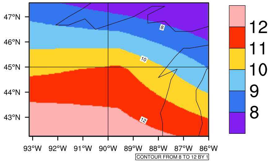
Yearly tasm max (c) In 2070-2079 GFDL-ESM2M RCP45 - Wisconsin
