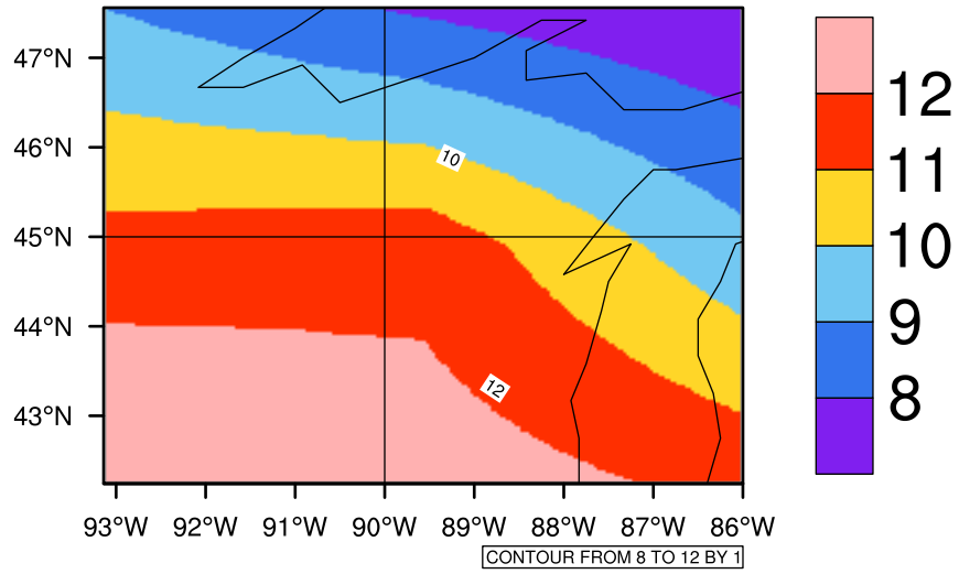
Yearly tasmax(c) In 2090-2099 GFDL-ESM2M RCP45 - Wisconsin
