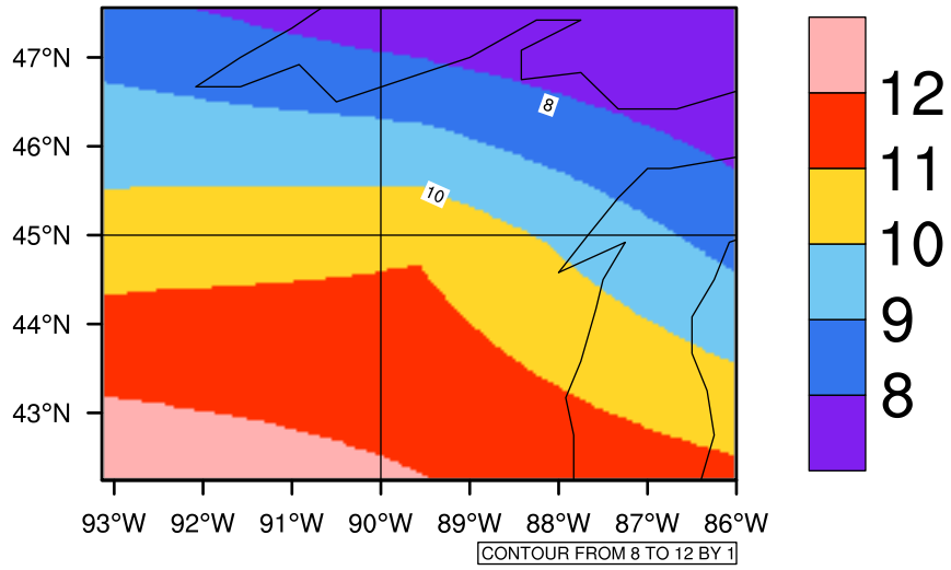
Yearly tasmax(c) In 2040-2049 GFDL-ESM2M RCP85 - Wisconsin
