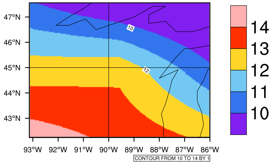
Yearly tasmx(c) In 2050-2059 GFDL-ESM2M RCP85 - Wisconsin
