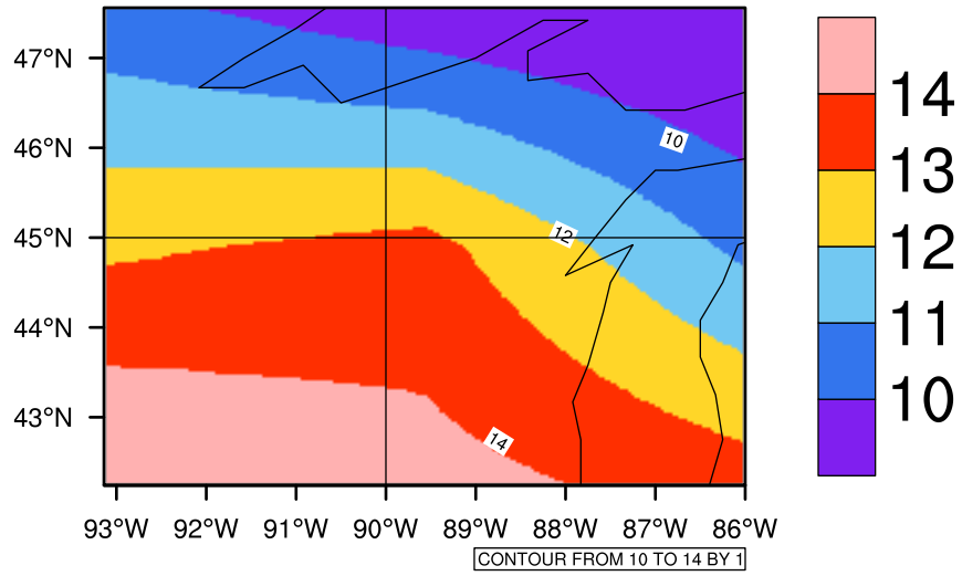
Yearly tasm max (c) In 2070-2079 GFDL-ESM2M RCP85 - Wisconsin
