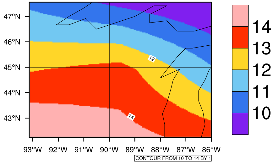
Yearly tasmax(c) In 2080-2089 GFDL-ESM2M RCP85 - Wisconsin
