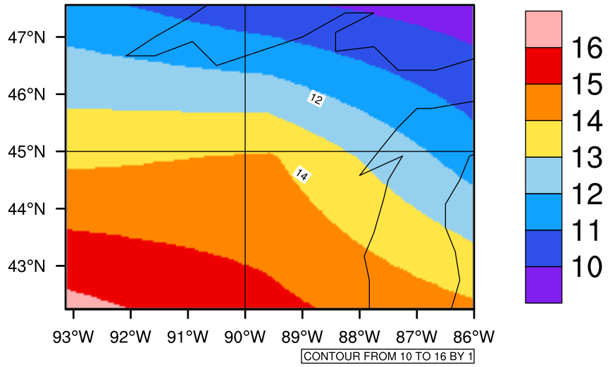
Yearly tasmx(c) In 2090-2099 GFDL-ESM2M RCP85 - Wisconsin
