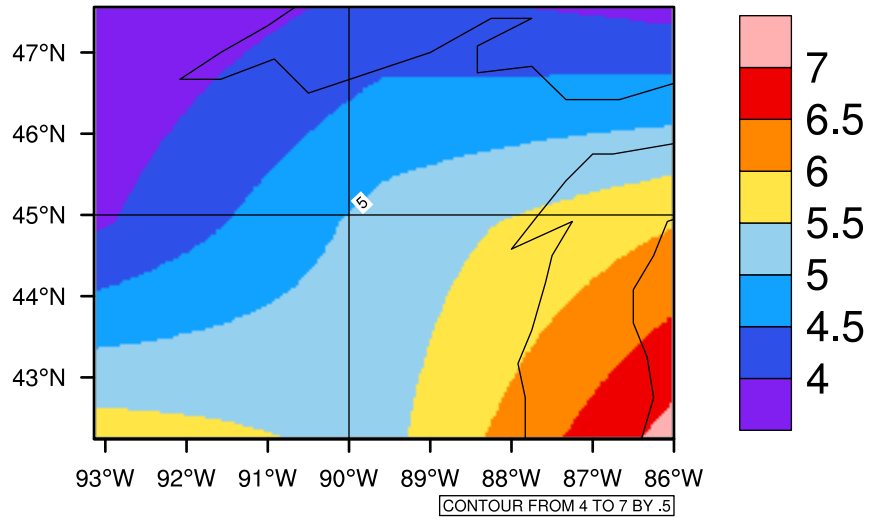
Yearly tasmin(c) In 2020-2029 GFDL-ESM2M RCP45 - Wisconsin
