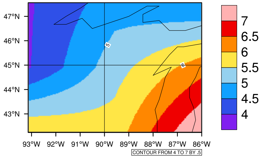
Yearly tasmin(c) In 2040-2049 GFDL-ESM2M RCP45 - Wisconsin
