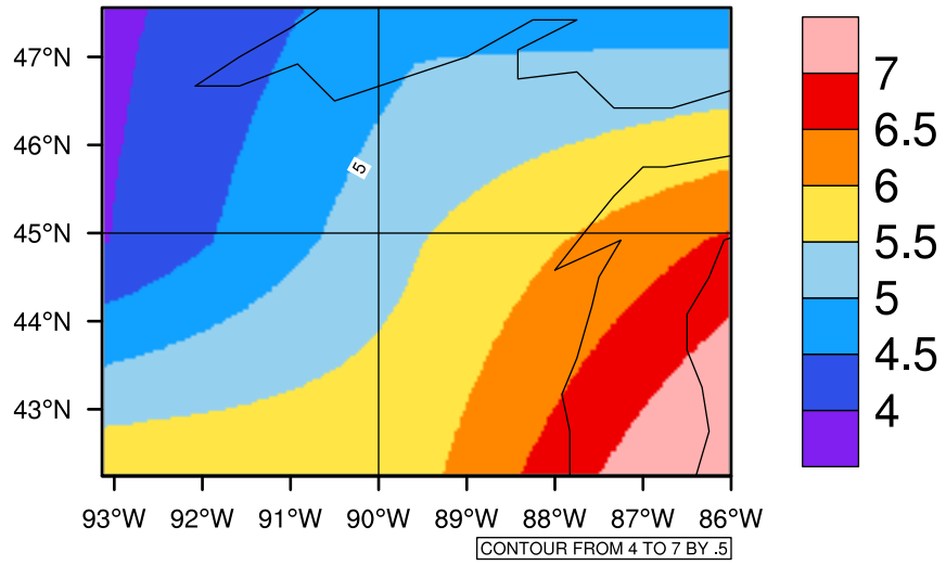
Yearly tasmin(c) In 2050-2059 GFDL-ESM2M RCP45 - Wisconsin
