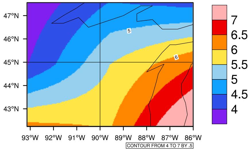
Yearly tasmin(c) In 2070-2079 GFDL-ESM2M RCP45 - Wisconsin
