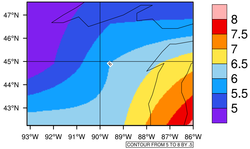
Yearly tasmin(c) In 2080-2089 GFDL-ESM2M RCP45 - Wisconsin
