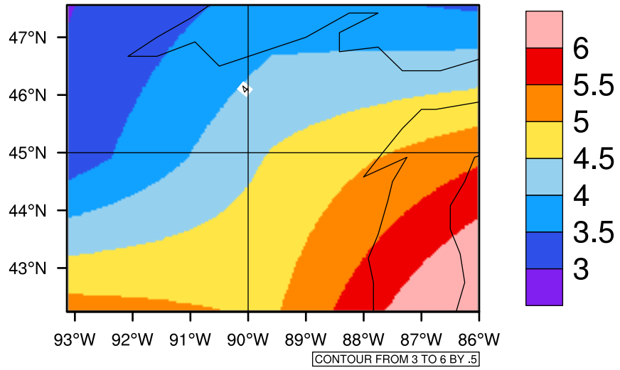
Yearly tasmin(c) In 2020-2029 GFDL-ESM2M RCP85 - Wisconsin
