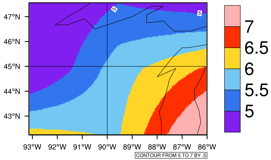
Yearly tasmin(c) In 2030-2039 GFDL-ESM2M RCP85 - Wisconsin
