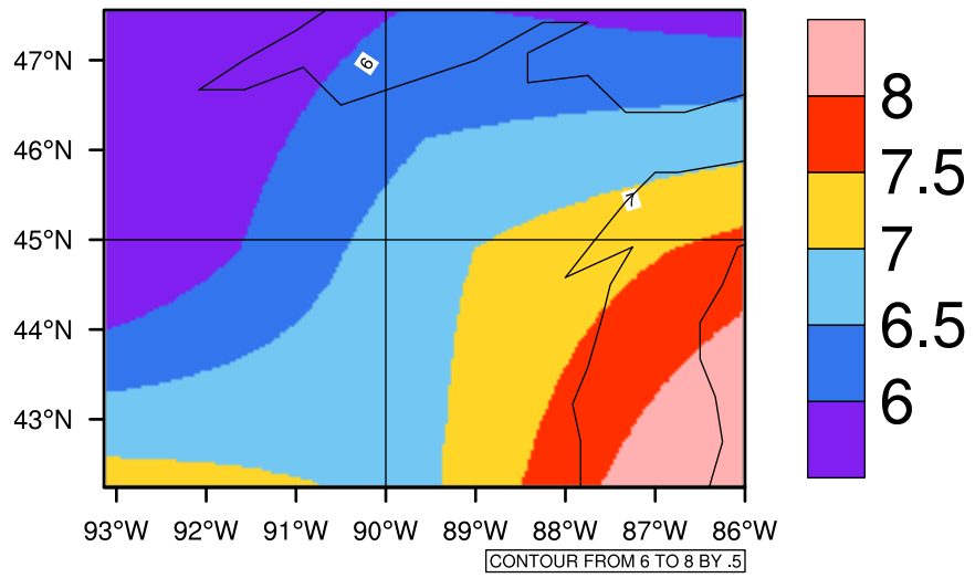
Yearly tasmin(c) In 2050-2059 GFDL-ESM2M RCP85 - Wisconsin
