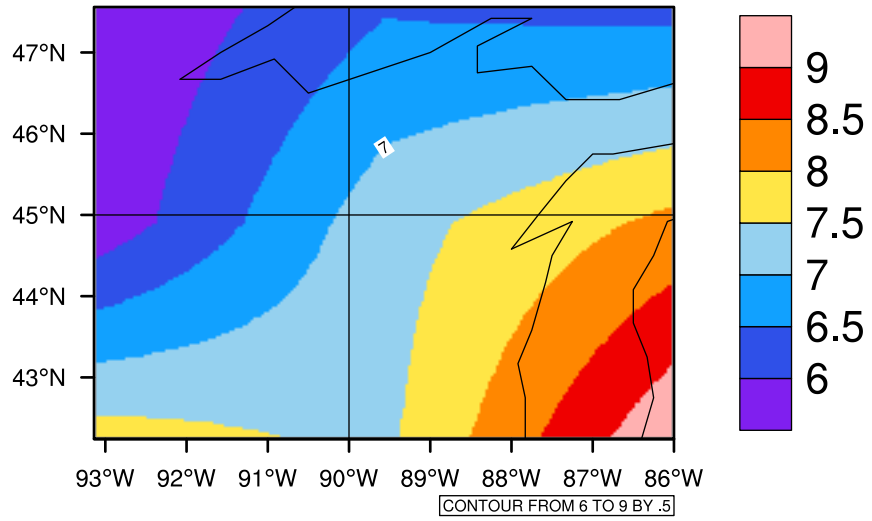
Yearly tasmin(c) In 2070-2079 GFDL-ESM2M RCP85 - Wisconsin
