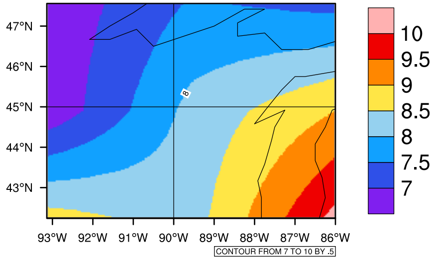
Yearly tasmin(c) In 2090-2099 GFDL-ESM2M RCP85 - Wisconsin
