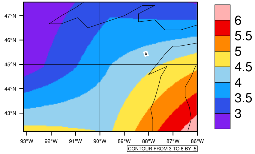
Yearly tasmin(c) In 1975-2005 GFDL-ESM2M historical - Wisconsin
