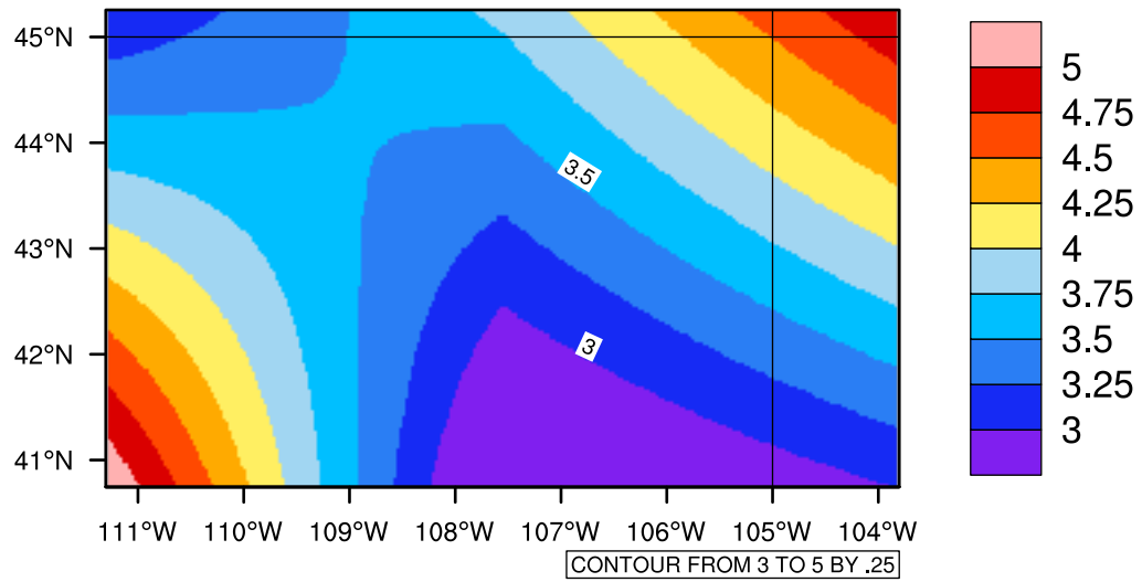
Yearly tas(c) In 2030-2039 GFDL-ESM2M RCP45 - Wyoming
