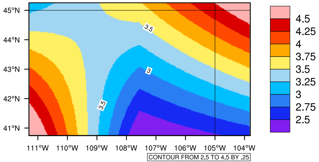
Yearly tas(c) In 2020-2029 GFDL-ESM2M RCP85 - Wyoming
