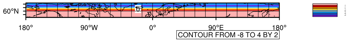
Yearly tasmin (c) In 2020-2029 MIROC4h RCP45 - Alaska
