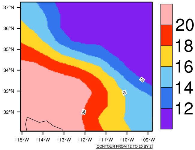
Yearly tas (c) In 1975-2005 MIROC4h historical - Arizona
