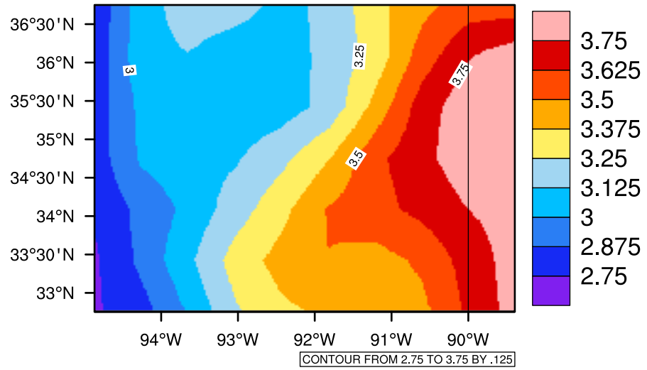
Yearly pr (mm/day) In 2020-2029 MIROC4h RCP45 - Arkansas
