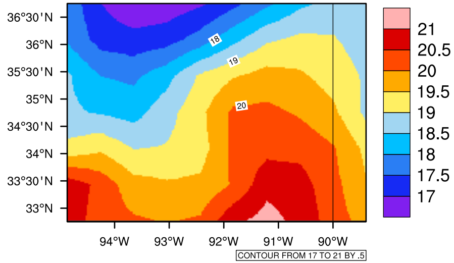
Yearly tas (c) In 2020-2029 MIROC4h RCP45 - Arkansas
