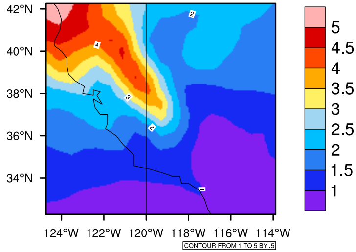
Yearly pr (mm/day) In 2020-2029 MIROC4h RCP45 - California
