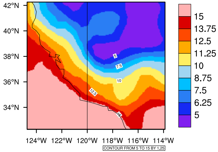
Yearly tasmin (c) In 2020-2029 MIROC4h RCP45 - California
