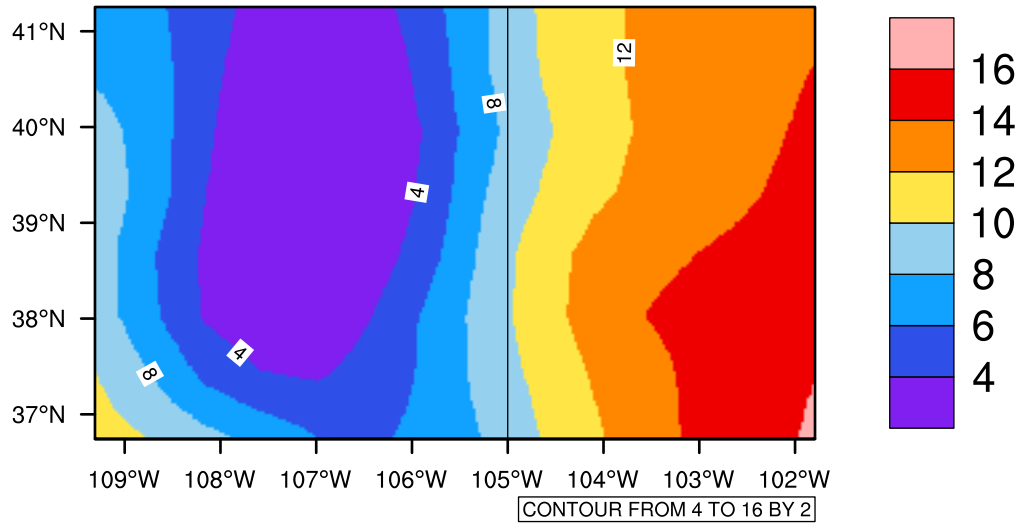
Yearly tas (c) In 2020-2029 MIROC4h RCP45 - Colorado
