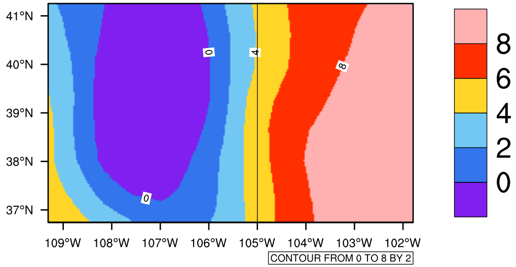
Yearly tasmin (c) In 2020-2029 MIROC4h RCP45 - Colorado
