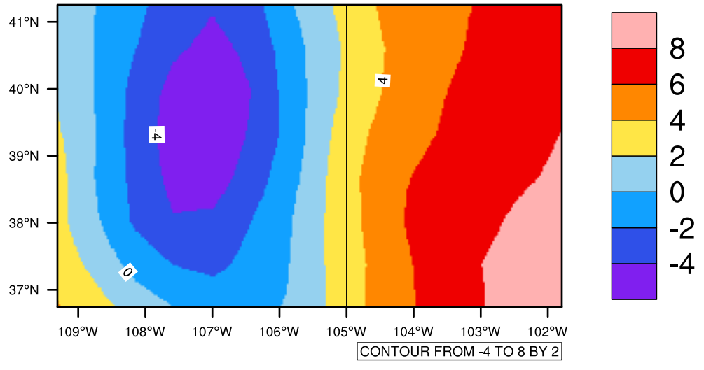
Yearly tasmin (c) In 1975-2005 MIROC4h historical - Colorado
