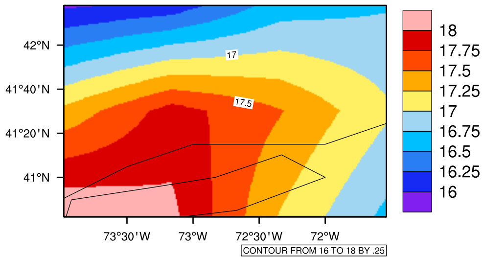
Yearly tasmax (c) In 2020-2029 MIROC4h RCP45 - Connecticut
