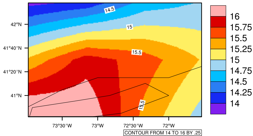
Yearly tasmax (c) In 1975-2005 MIROC4h historical - Connecticut
