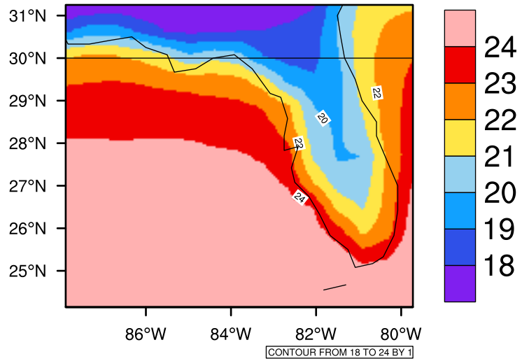
Yearly tasmin (c) In 2020-2029 MIROC4h RCP45 - Florida
