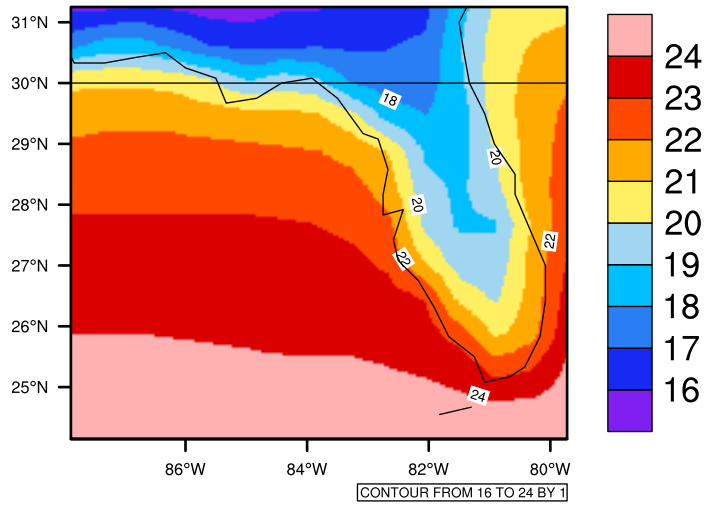
Yearly tasmin (c) In 1975-2005 MIROC4h historical - Florida
