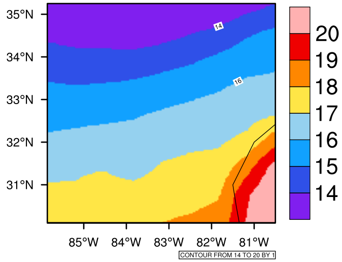
Yearly tasmin (c) In 2020-2029 MIROC4h RCP45 - Georgia
