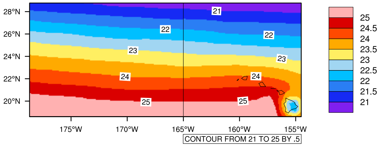
Yearly tasmin (c) In 2020-2029 MIROC4h RCP45 - Hawaii
