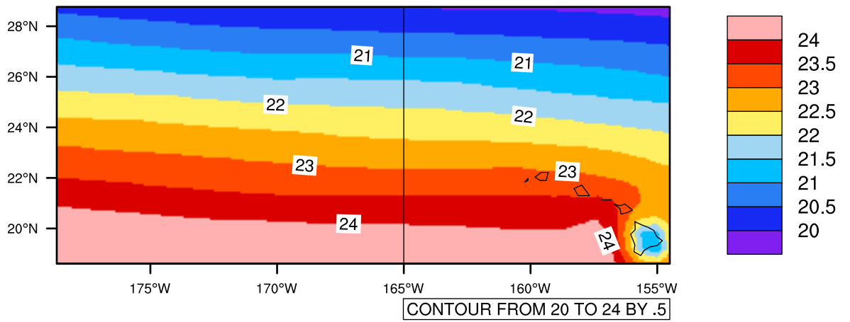
Yearly tasmin (c) In 1975-2005 MIROC4h historical - Hawaii
