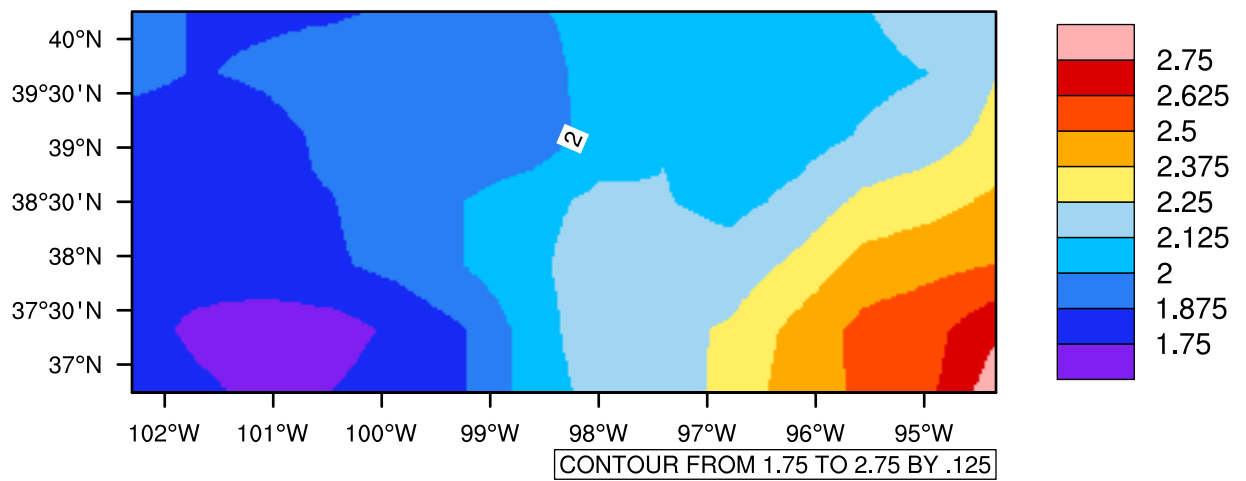
Yearly pr (mm/day) In 2020-2029 MIROC4h RCP45 - Kansas
