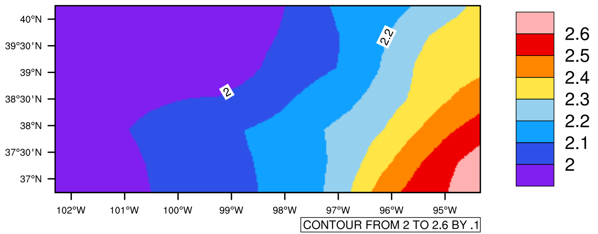
Yearly pr (mm/day) In 1975-2005 MIROC4h historical - Kansas
