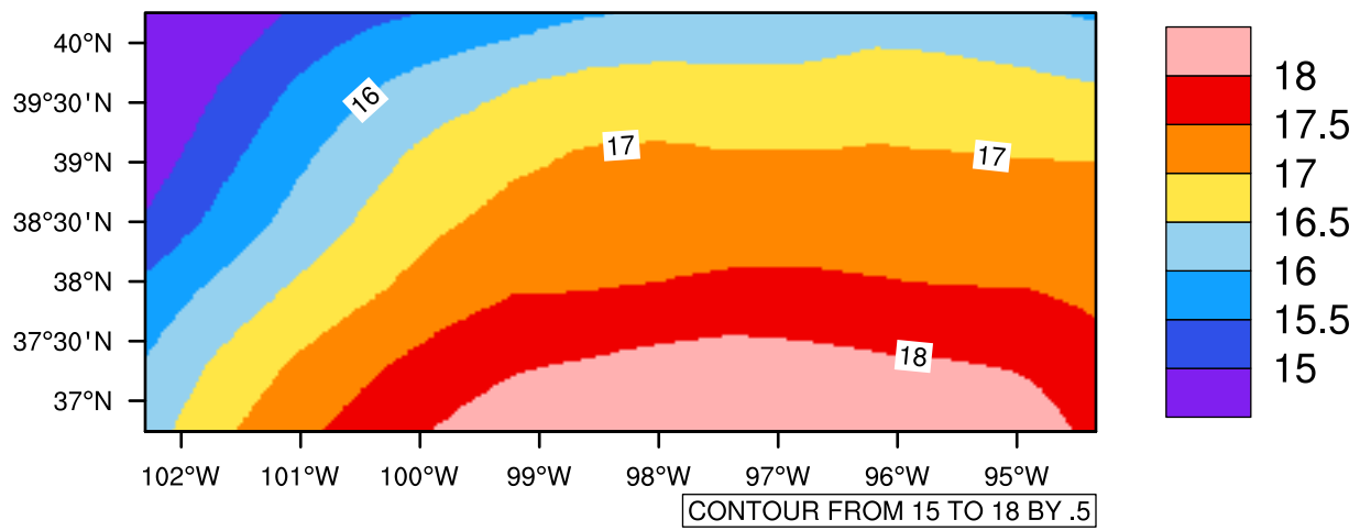
Yearly tas (c) In 2020-2029 MIROC4h RCP45 - Kansas
