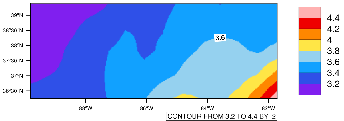
Yearly pr (mm/day) In 1975-2005 MIROC4h historical - Kentucky
