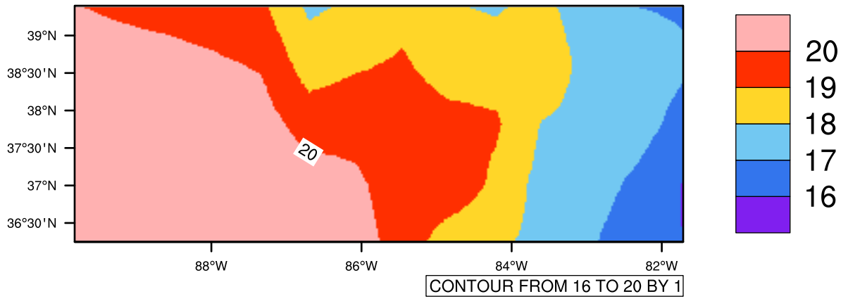
Yearly tasmax (c) In 1975-2005 MIROC4h historical - Kentucky
