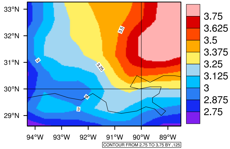
Yearly pr (mm/day) In 2020-2029 MIROC4h RCP45 - Louisiana
