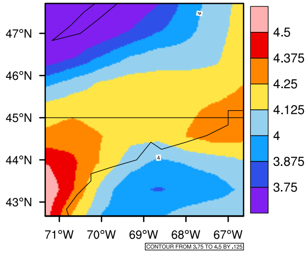
Yearly pr (mm/day) In 2020-2029 MIROC4h RCP45 - Maine
