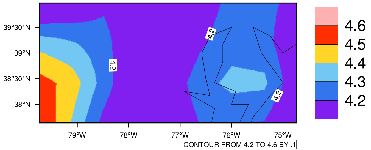
Yearly pr (mm/day) In 2020-2029 MIROC4h RCP45 - Maryland
