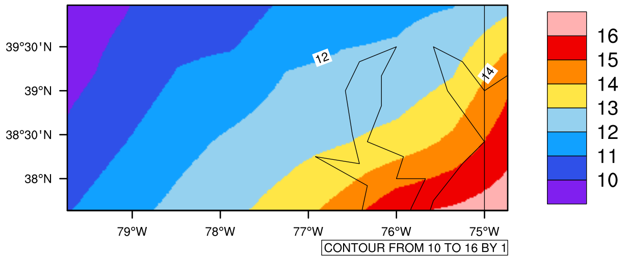
Yearly tasmin (c) In 2020-2029 MIROC4h RCP45 - Maryland
