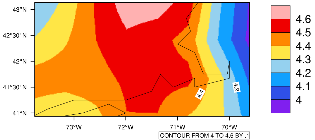
Yearly pr (mm/day) In 2020-2029 MIROC4h RCP45 - Massachusetts
