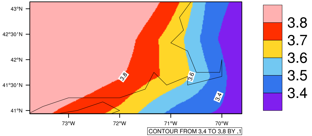
Yearly pr (mm/day) In 1975-2005 MIROC4h historical - Massachusetts
