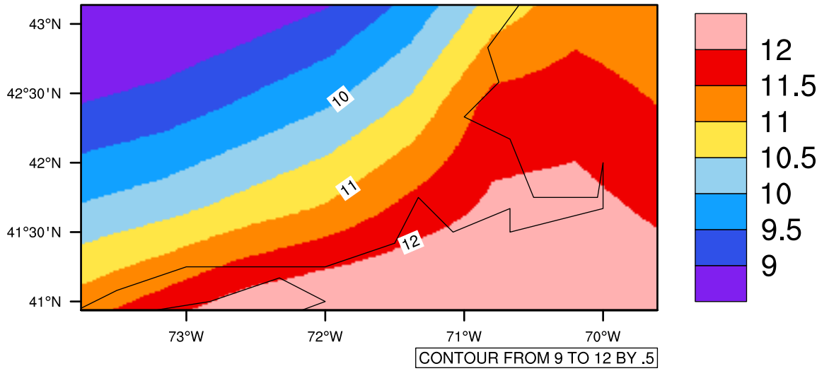
Yearly tas (c) In 1975-2005 MIROC4h historical - Massachusetts
